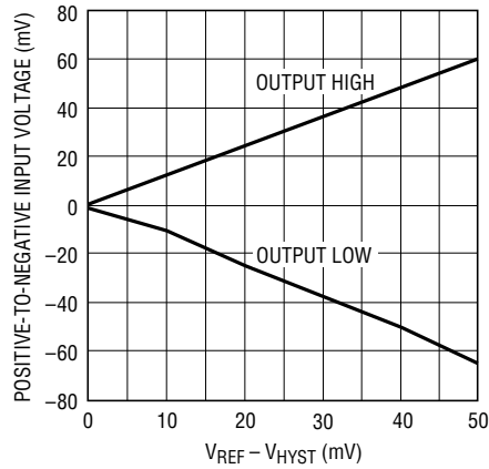
Hysteresis Control
